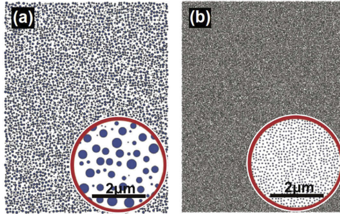
Fig. 2. Modeling light propagation through computational representations of: (a) sclera and (b) cornea. In a 22\ \mu\text{m} \times 30\ \mu\text{m} region, the scattering medium consists of: (a) sclera: 6000 mixed-size collagen fibrils with diameter ranging from 29.74 nm to 297.4 nm randomly positioned in space, (b) cornea: 86775 uniform collagen fibrils with a diameter of 29.74 nm randomly positioned in space. The refractive index of the collagen fibrils is n_c = 1.504 immersed in extrafibrillar substance with a refractive index of: n_b = 1.345 .
